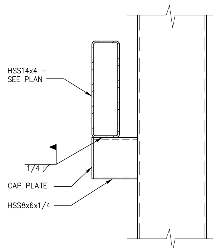
STRINGER SUPPORT CONNECTION
