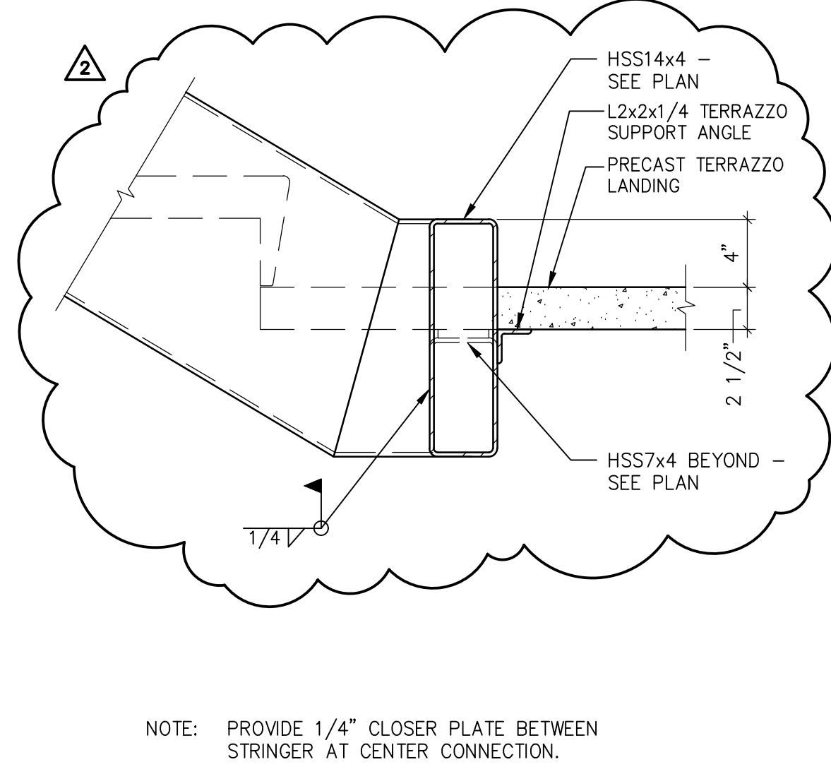
STRINGER TO TUBE CONNECTION
