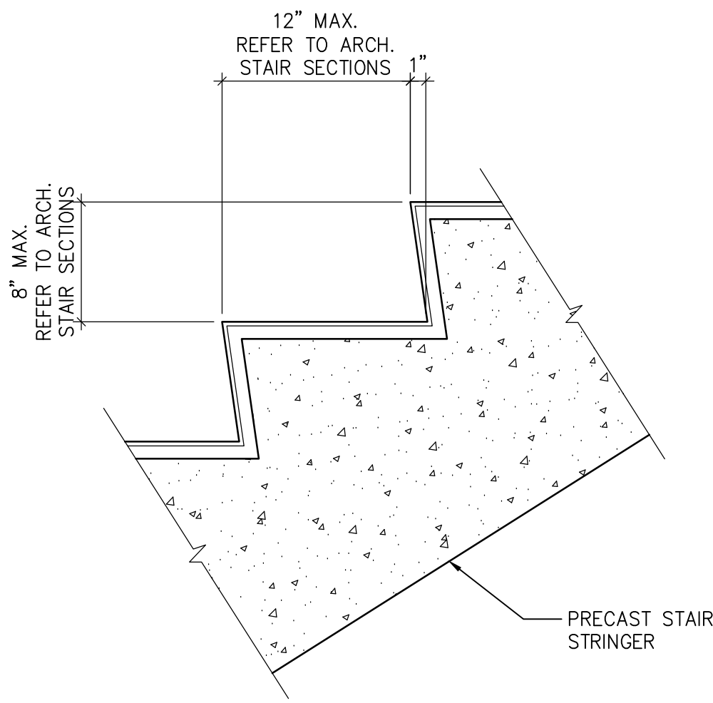
PRECAST CONCRETE TREAD & RISER DETAIL
