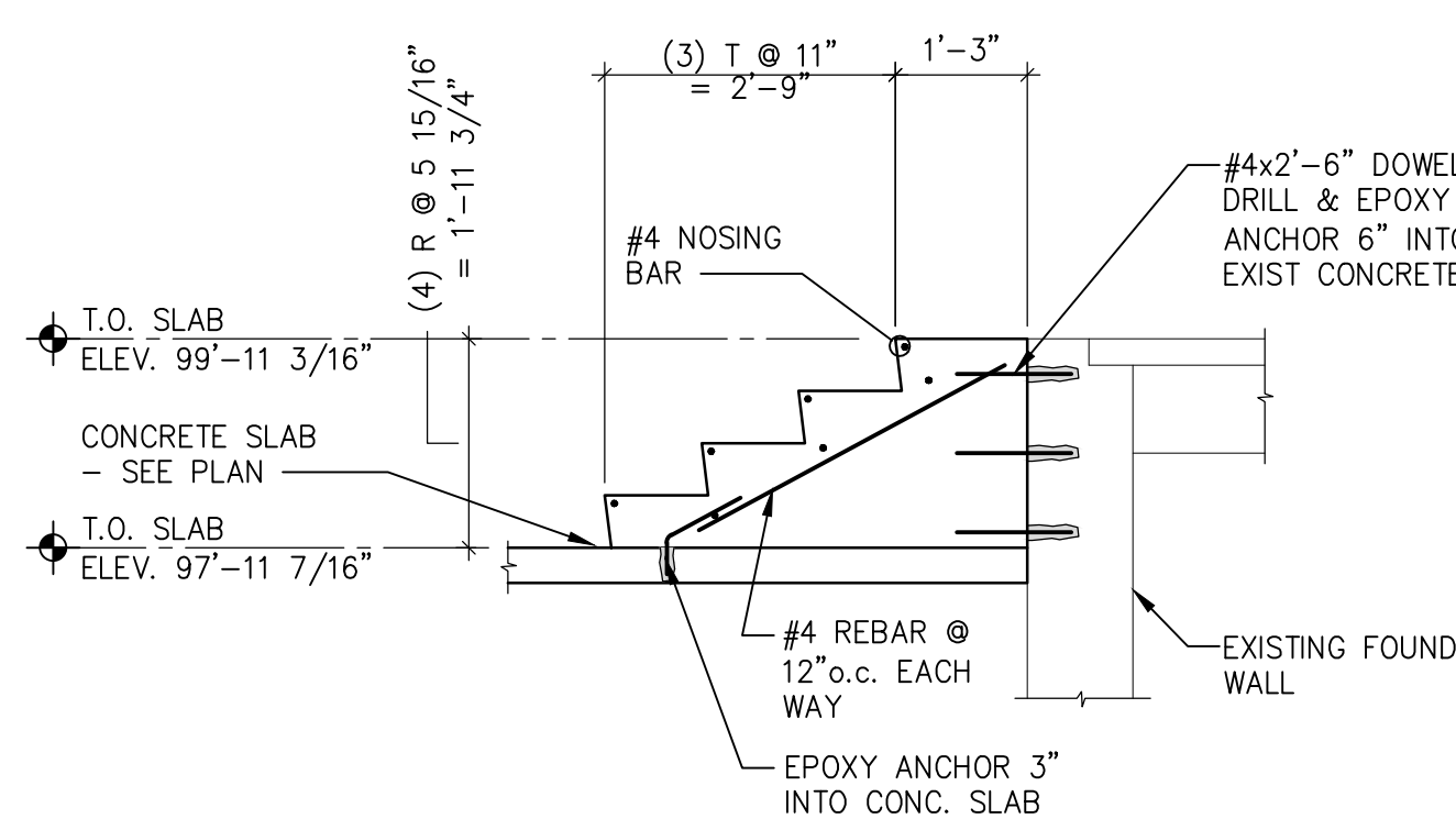
CONCRETE STAIR SECTION
