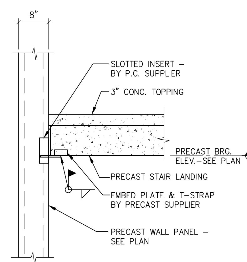
PRECAST STAIR TO PRECAST WALL
