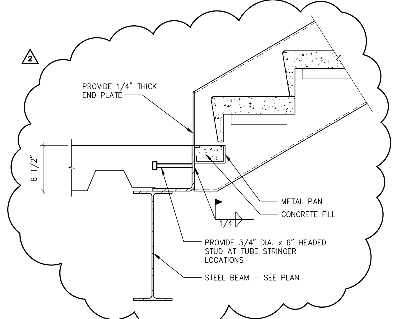
STAIR PURLIN TO FLOOR BEAM
