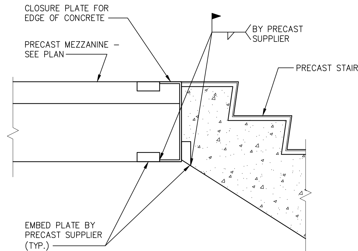
PRECAST STAIR TO FLOOR
