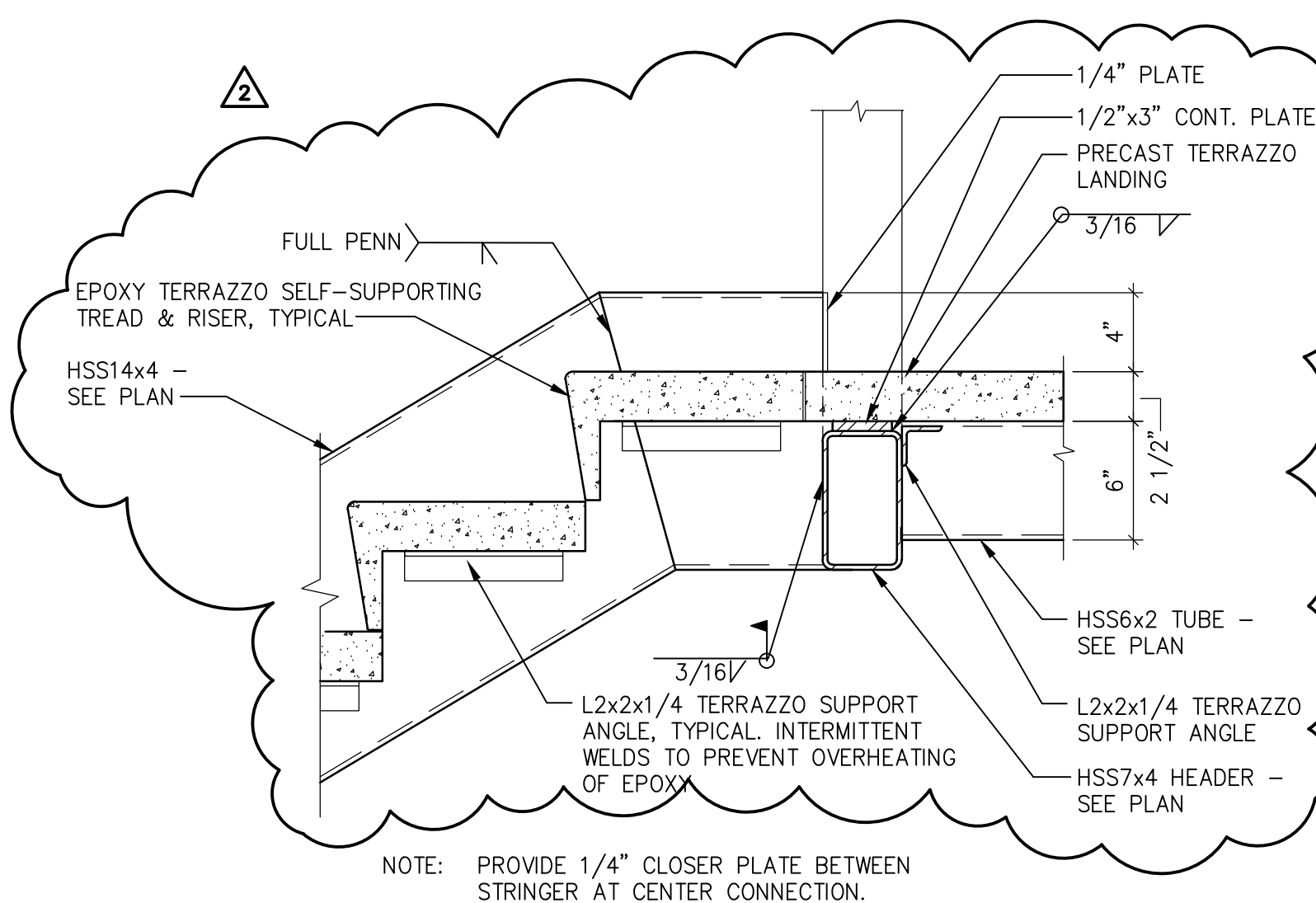
STRINGER TO TUBE CONNECTION
