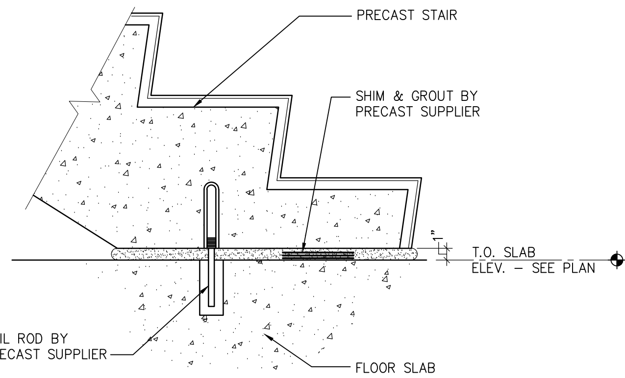
PRECAST STAIR TO FLOOR
