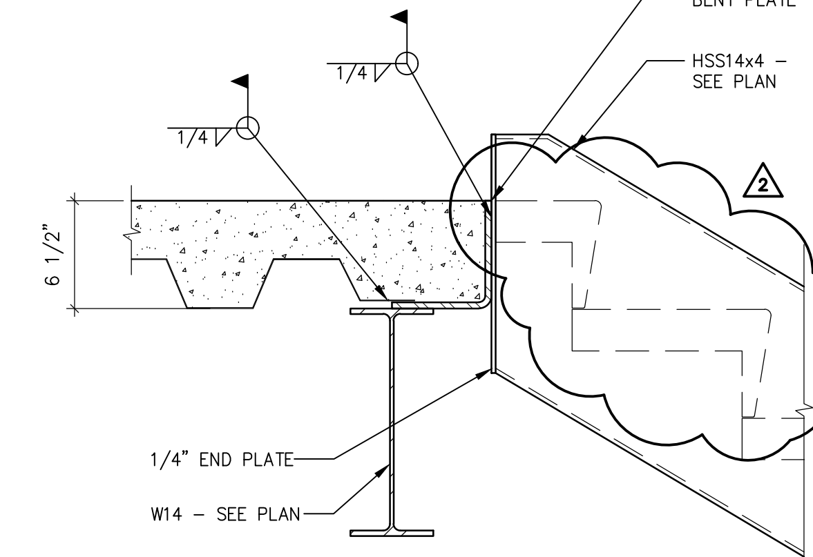
STAIR PURLIN TO FLOOR BEAM
