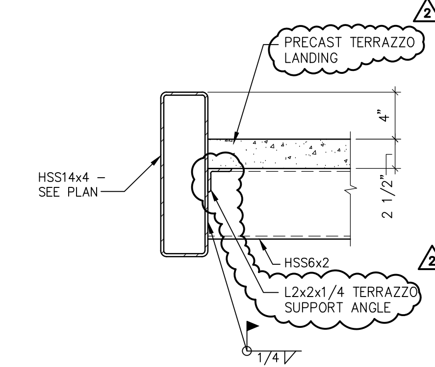
HANGER CONNECTION
