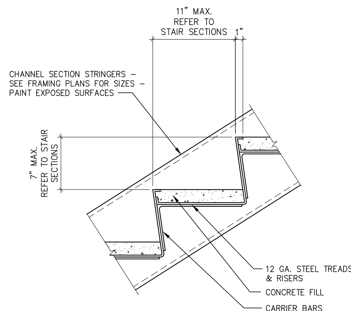
TREAD AND RISER DETAIL
