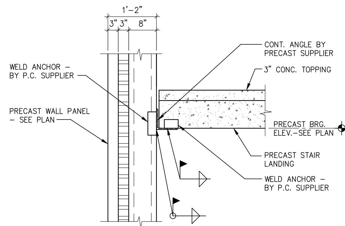
PRECAST STAIR TO PRECAST WALL
