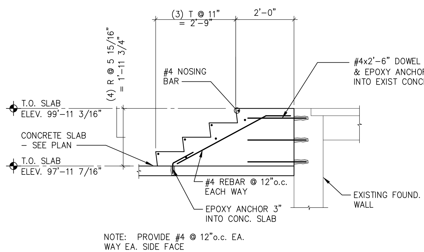
CONCRETE STAIR SECTION
