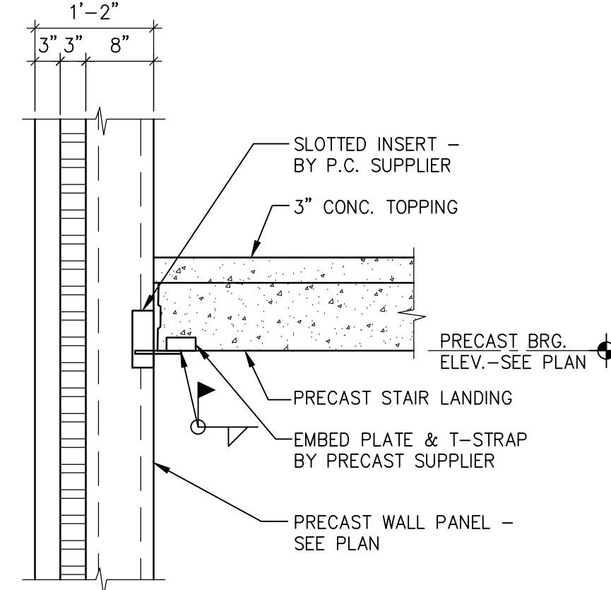
PRECAST STAIR TO PRECAST WALL
