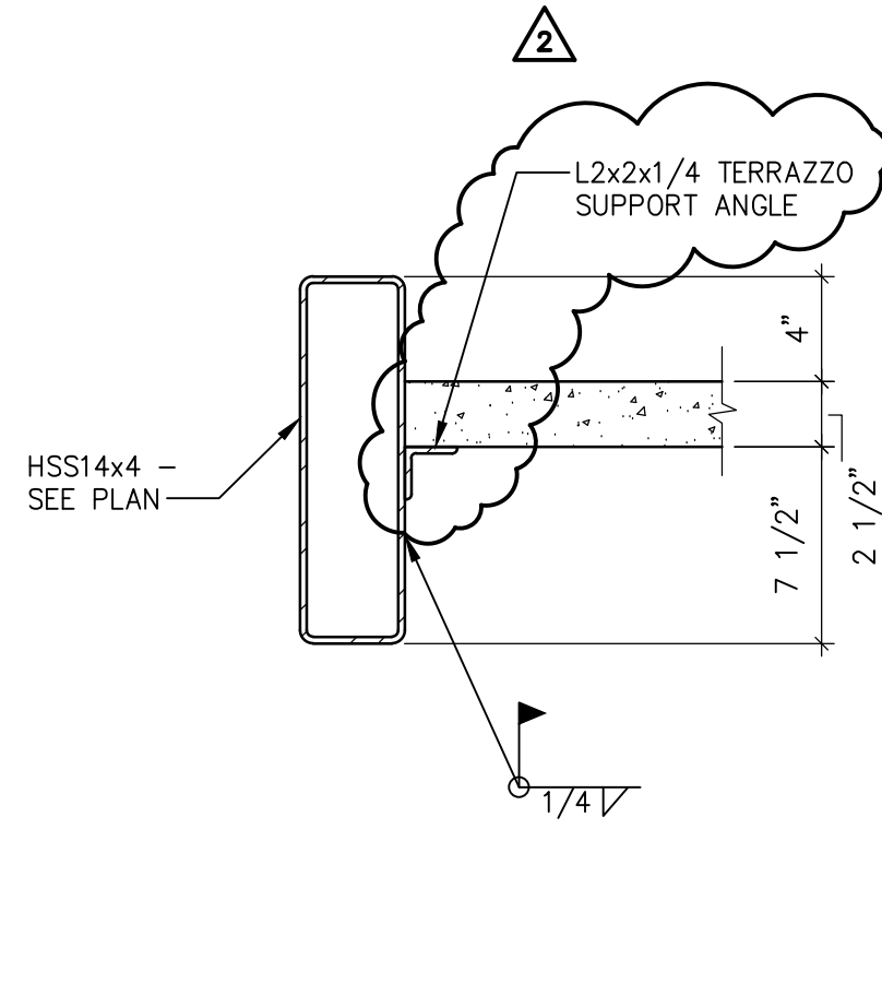
SLAB TO STAIR STRINGER
