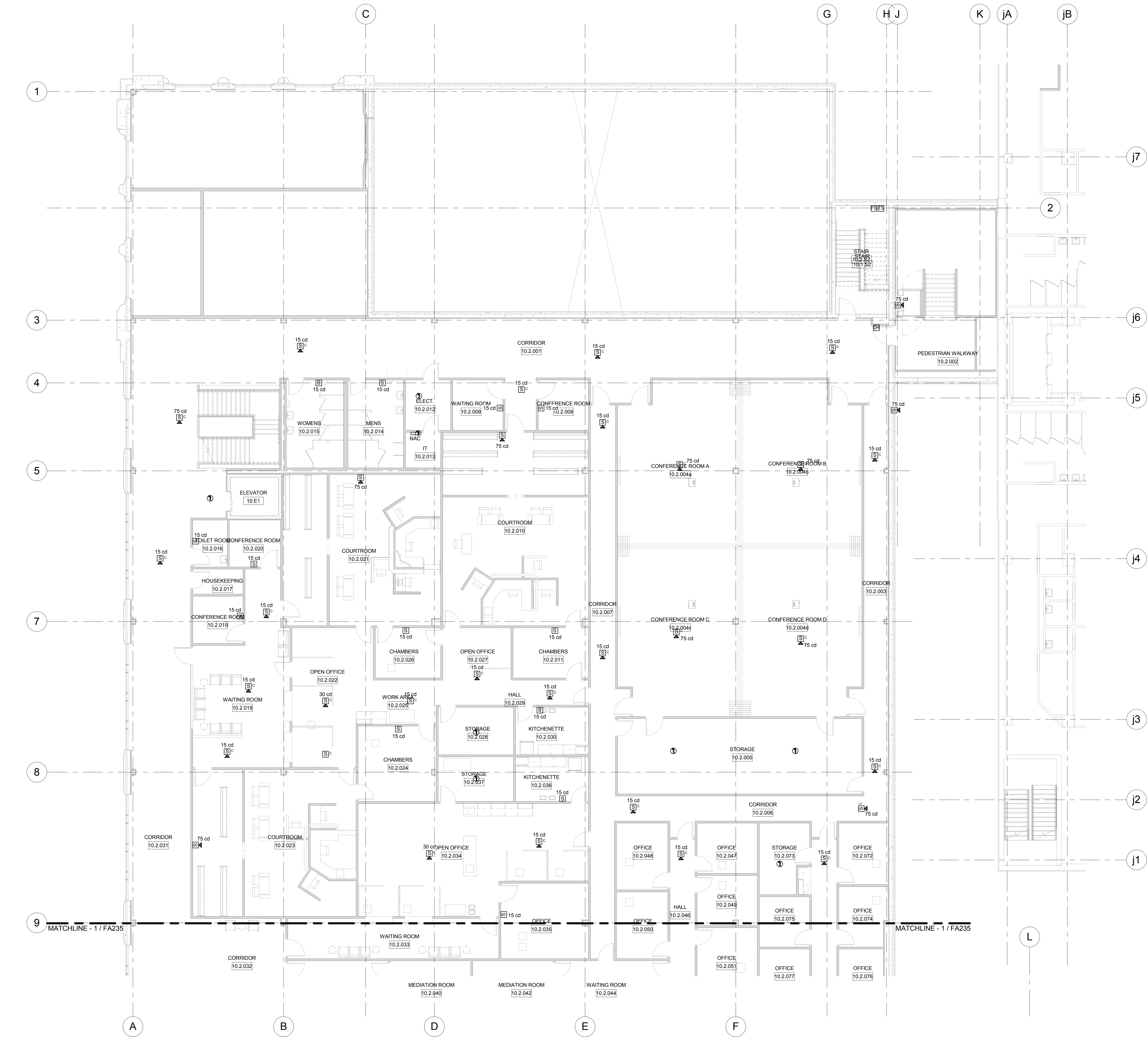
1 LEVEL 805.00 FIRE ALARM SYSTEM PLAN-OCAC NORTH Scale: 1/8" = 1'-0"
