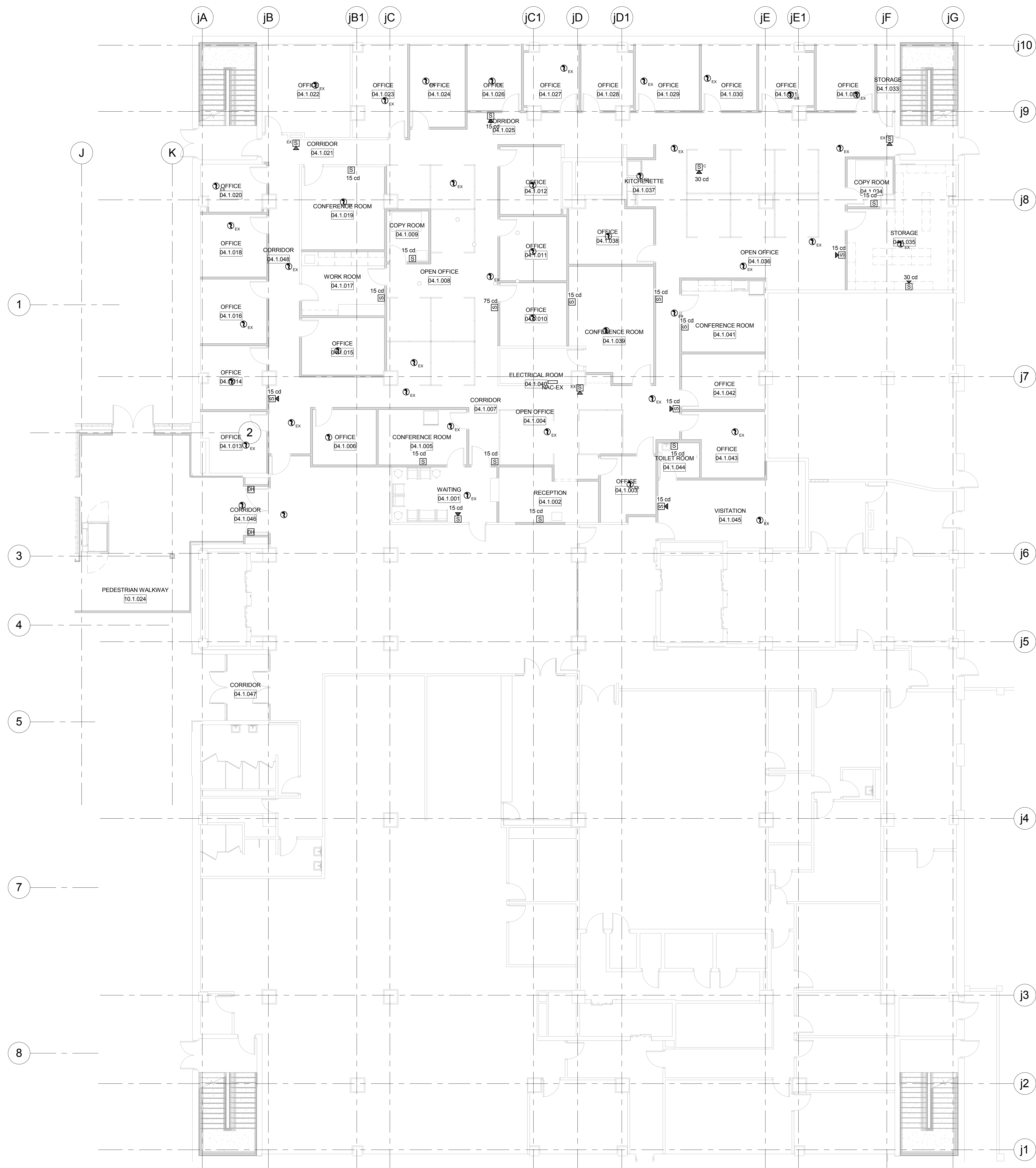
1 LEVEL 790.00 FIRE ALARM SYSTEM PLAN-JUSTICE CENTER
