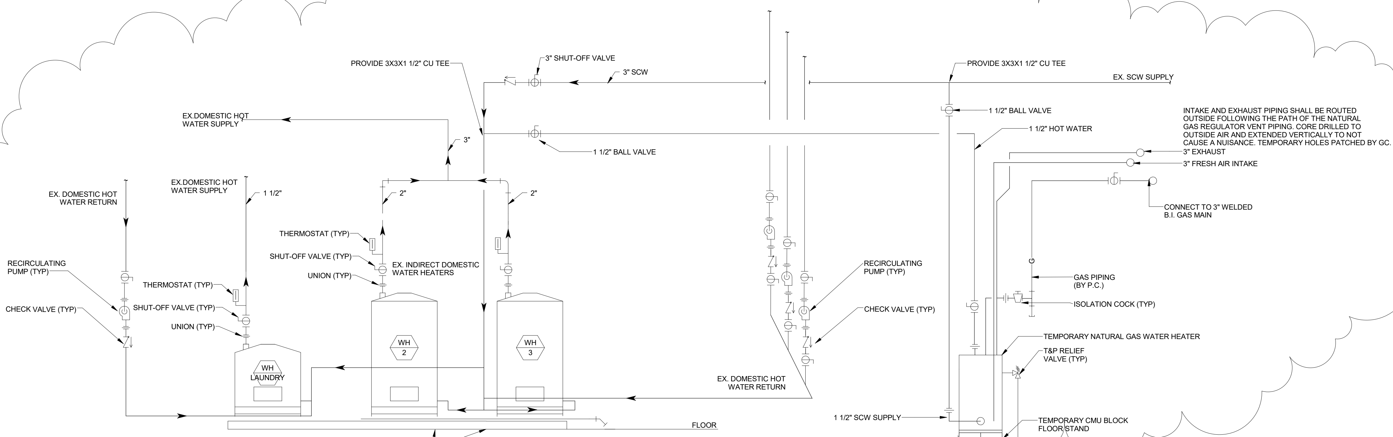
WATER HEATER PIPING DETAIL - JUSTICE CENTER NOT TO SCALE
