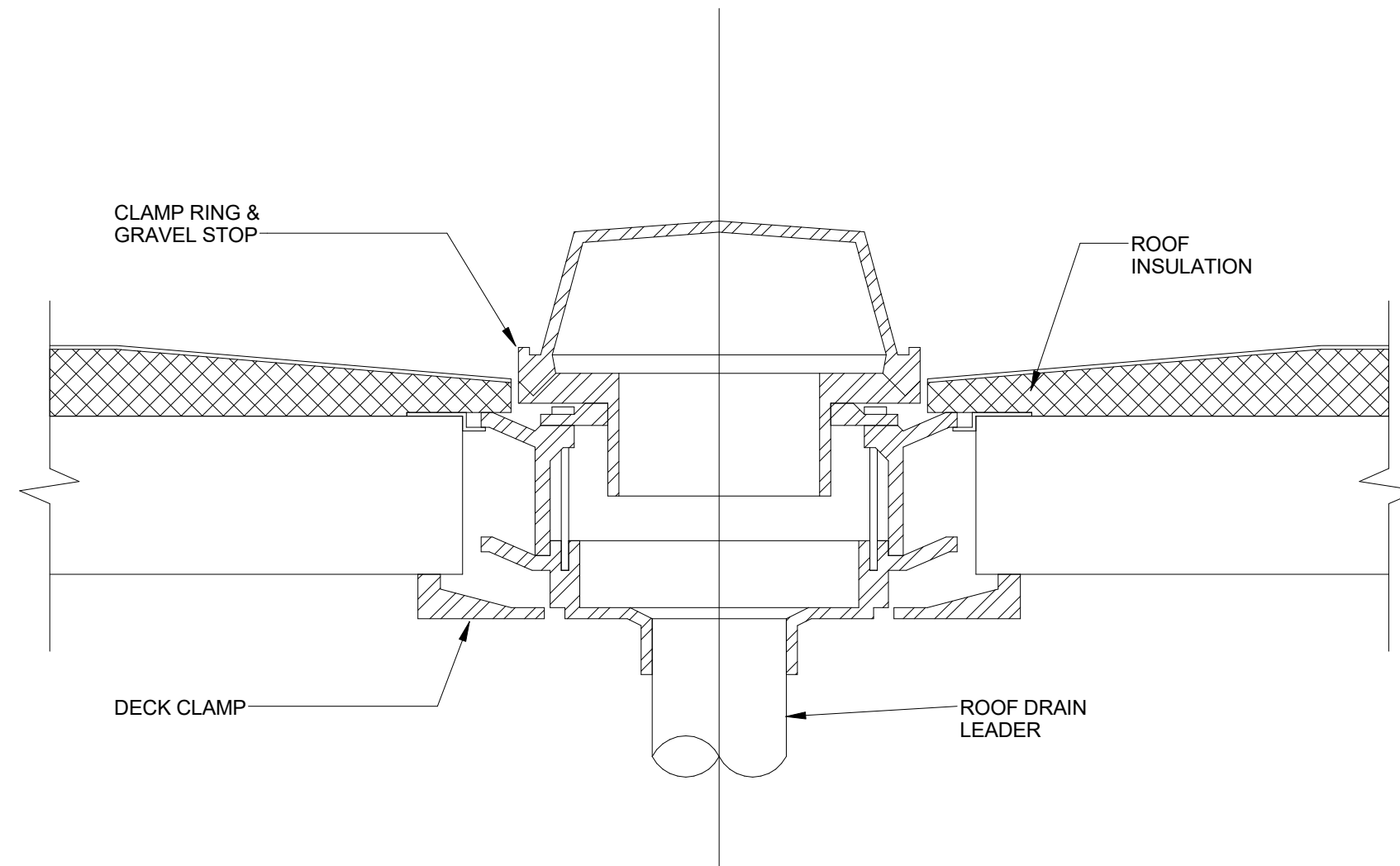
2 ROOF DRAIN DETAIL P501 1/4" = 1'-0" 0 4' 8' 16'
