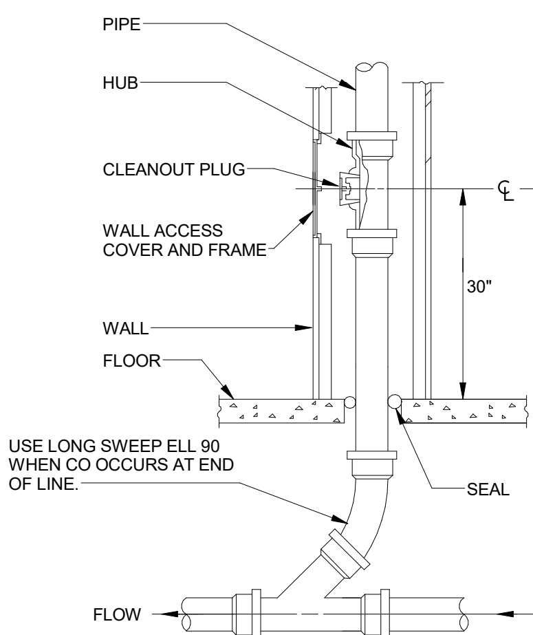
5 WALL CLEAN OUT DETAIL P501 1/8" = 1'-0" 0 4' 8' 16'
