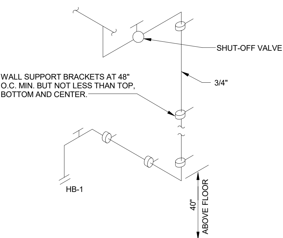
3 INTERIOR HOSE BIBB PIPING RISER P501 1/8" = 1'-0" 0 4' 8' 16'
