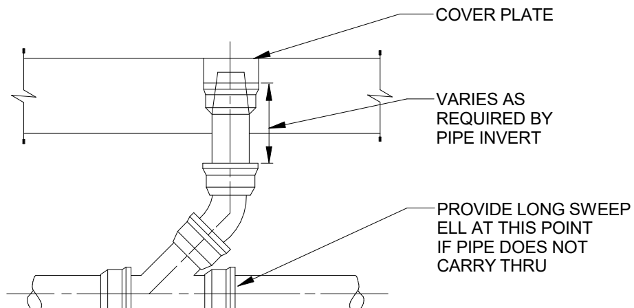
8 CLEAN OUT AND PLUGGED RISER P501 1/8" = 1'-0" 0 4' 8' 16'
