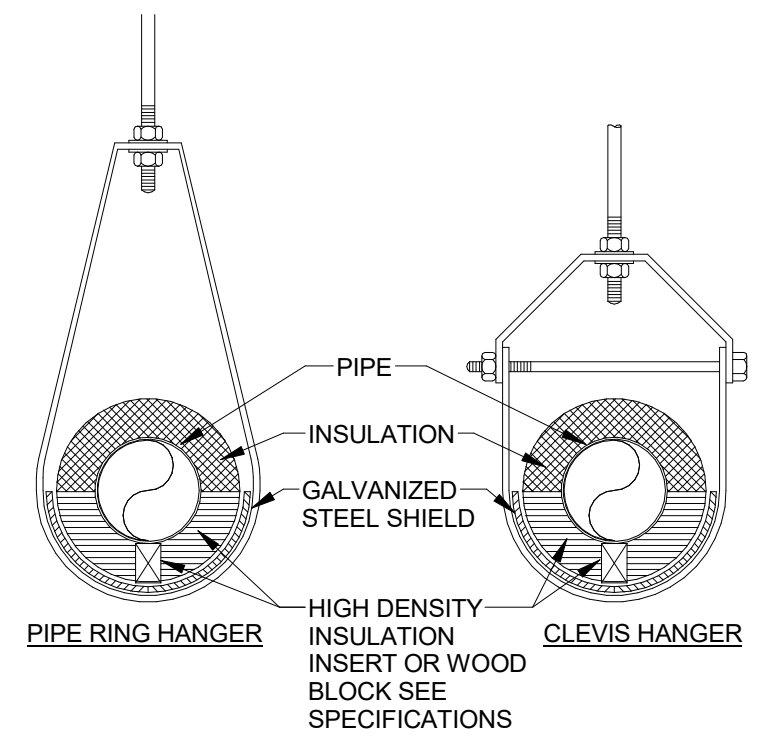
4 INSULATED PIPE AT HANGER DETAIL P501 1/8" = 1'-0" 0 4' 8' 16'
