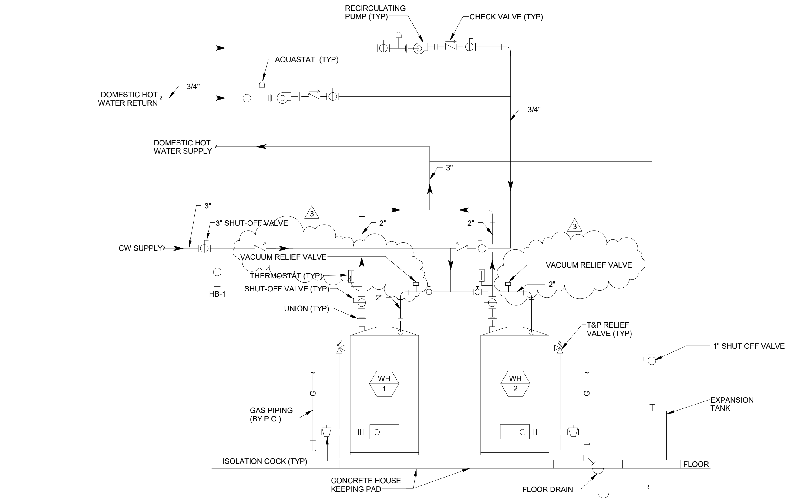
1 WATER HEATER PIPING DETAIL - TWO HEATERS P501 1/8" = 1'-0" 0 4' 8' 16'
