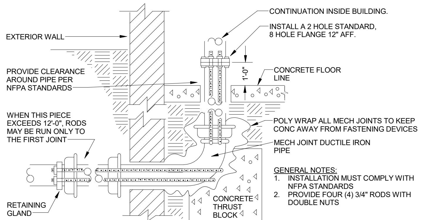
8 WATER SERVICE LINE EXTENSION DETAIL P501 NO SCALE 0 4' 8' 16'
