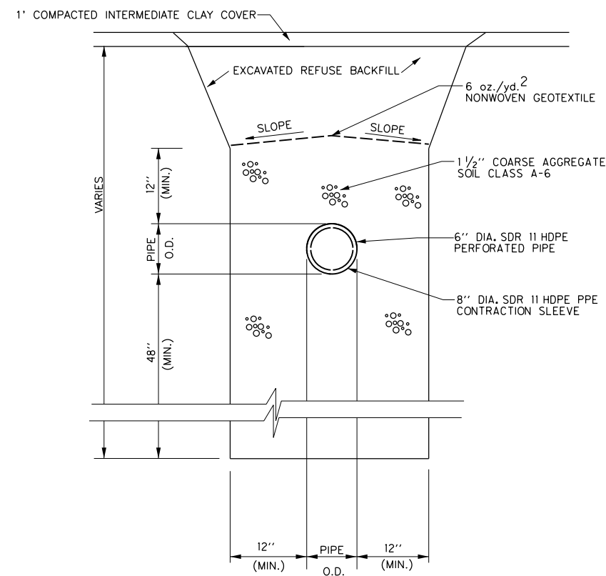
1' COMPACTED INTERMEDIATE CLAY COVER EXCAVATED REFUSE BACKFILL 6 oz./yd. 2 NONWOVEN GEOTEXTILE SLOPE 1 1/2" COARSE AGGREGATE SOIL CLASS A-6 12" (MIN.) PIPE O.D. 12" (MIN.) 6" DIA. SDR 11 HDPE PERFORATED PIPE 12" (MIN.) PIPE O.D. 12" (MIN.) VARIABLES (4.5' TO 7')
