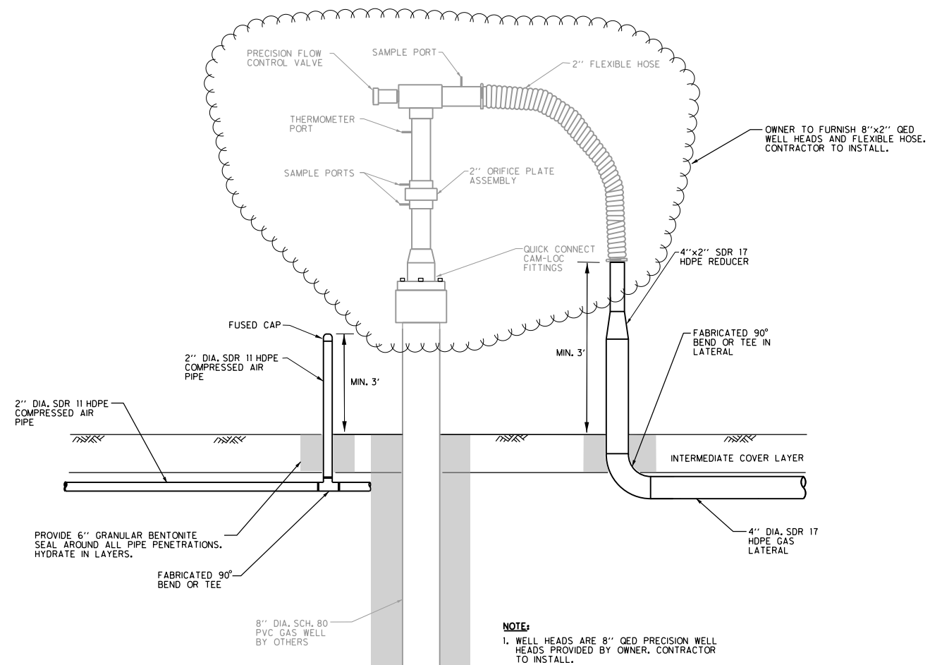
5 TYPICAL VERTICAL GAS WELL HEAD INSTALLATION 8 NOT TO SCALE
