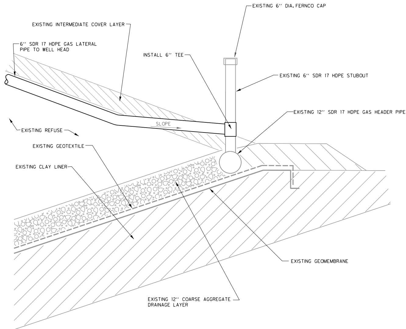
1 TYPICAL CONNECTION TO EXISTING STUBOUT 8 NOT TO SCALE
